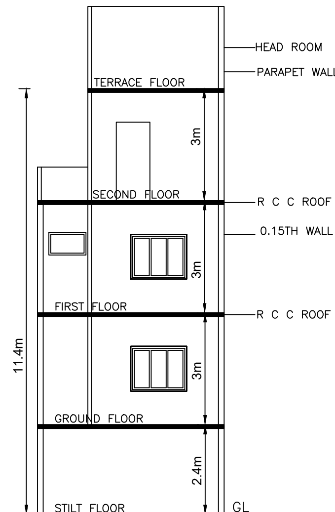
SECTION @ X-X
